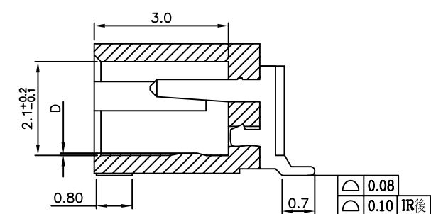
SECTION X-X
